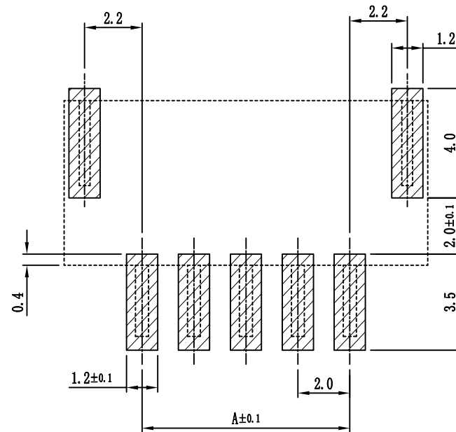
PCB PATTERN LAYOUT
